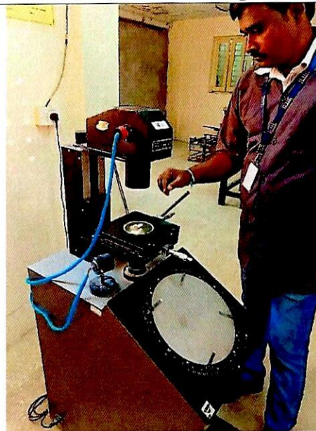
Profile Projector
